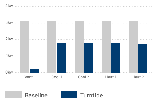
Savings by Mode (All motors)
