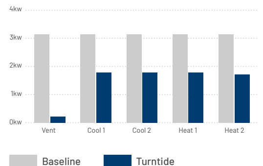
Savings by Mode (All motors)
